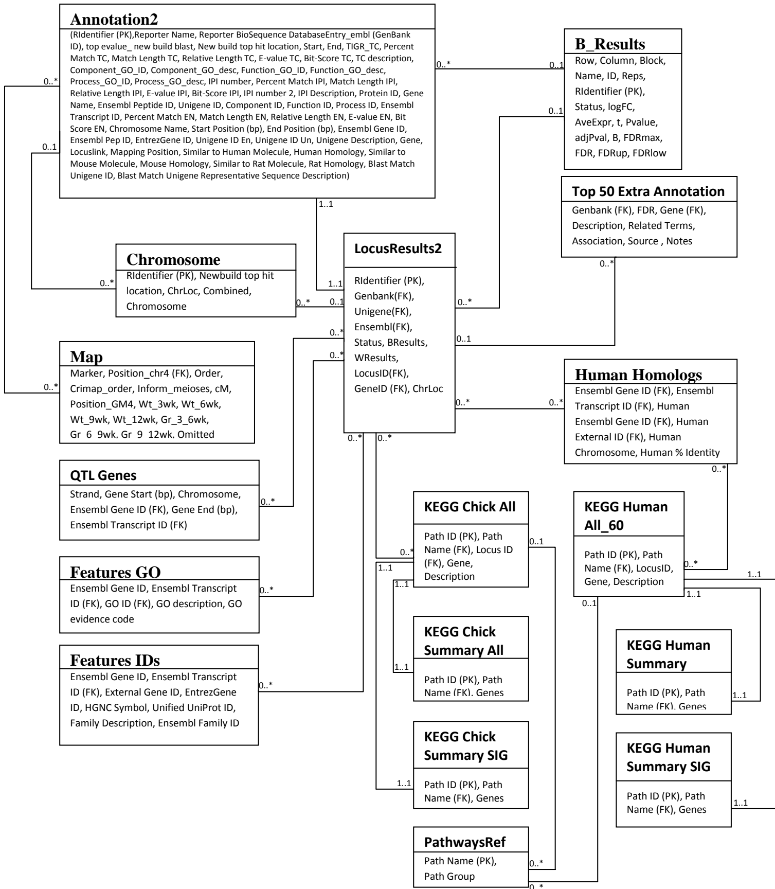
Figure 4.2 Entity Relationship Diagram of the Targeted Genetical Genomics Database.
